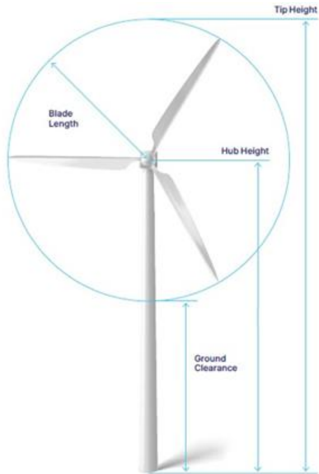
Figure 2 Wind turbine generator measurements (TransAlta, 2024)
